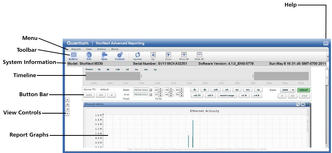
Figure 7 Report Window
