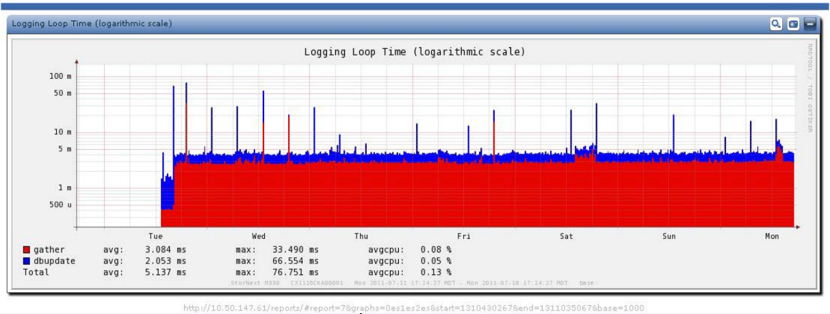
Figure 8 URL Reference
